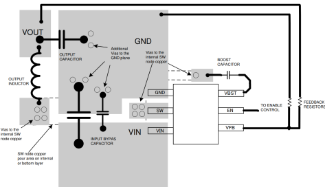
Figure 7-16. Board Layout
